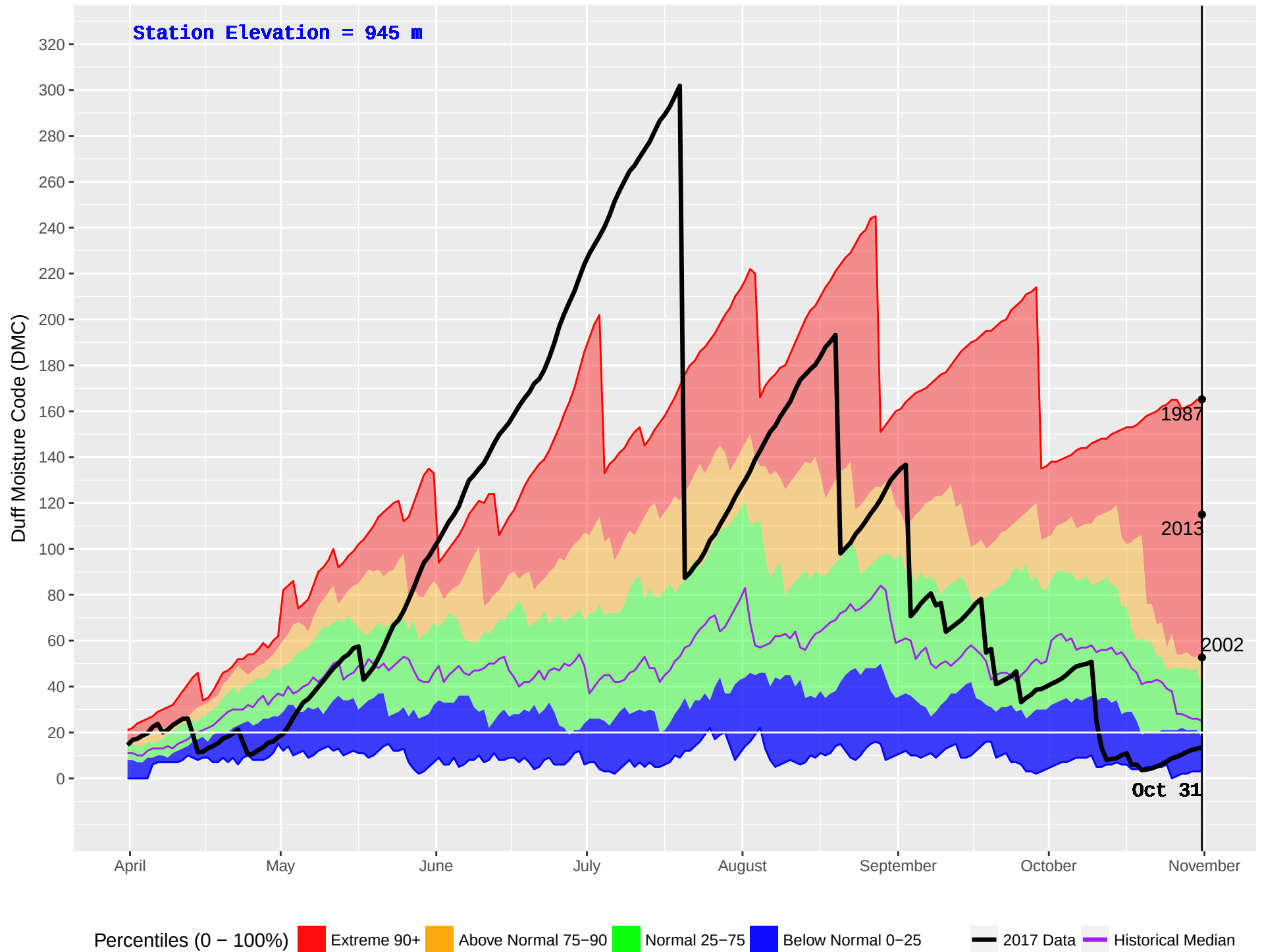
TATLA LAKE HUB (208) : Historical (1980–2016) and Current (2017) Noon Duff Moisture Code (DMC)
