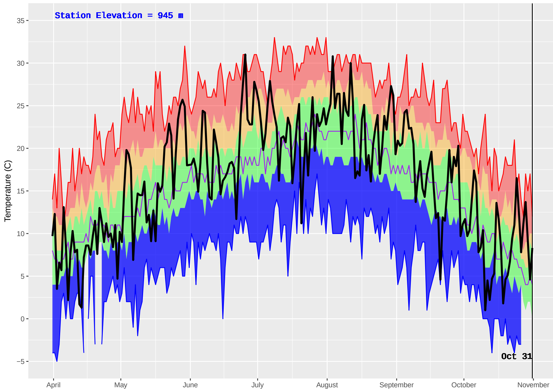
TATLA LAKE HUB (208) : Historical (1980–2016) and Current (2017) Noon Temperature
